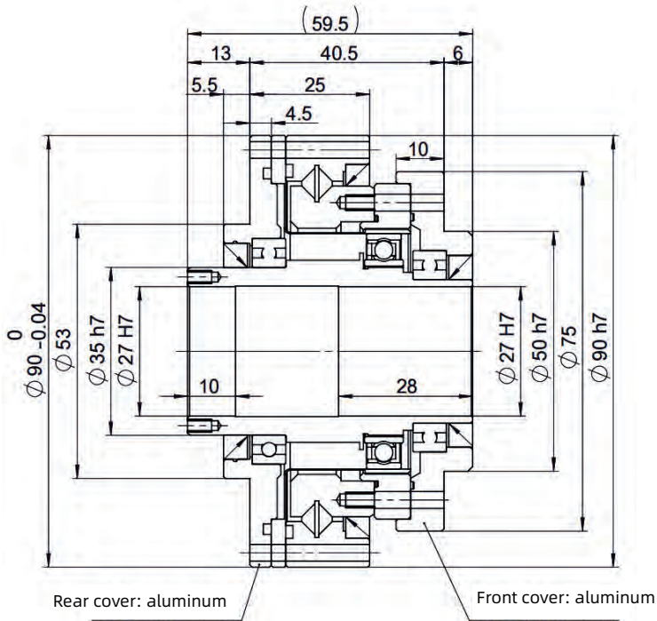
Full-section front view
