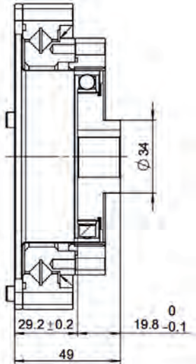
Wave Generator Reverse Installation Dimensions
