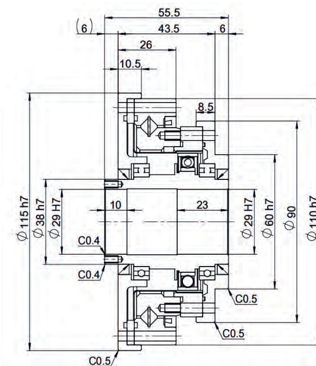
Full-section front view
