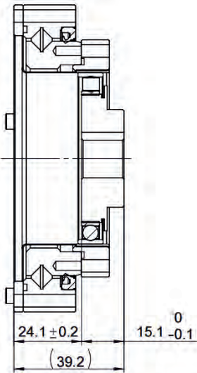
Wave Generator Reverse Installation Dimensions
