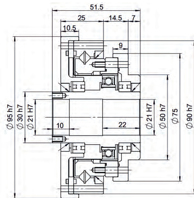
Full-section front view
