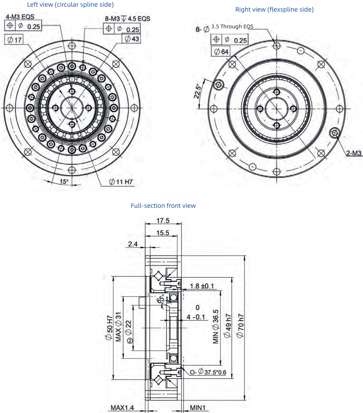
PMHD-III Series Structural Diagram
