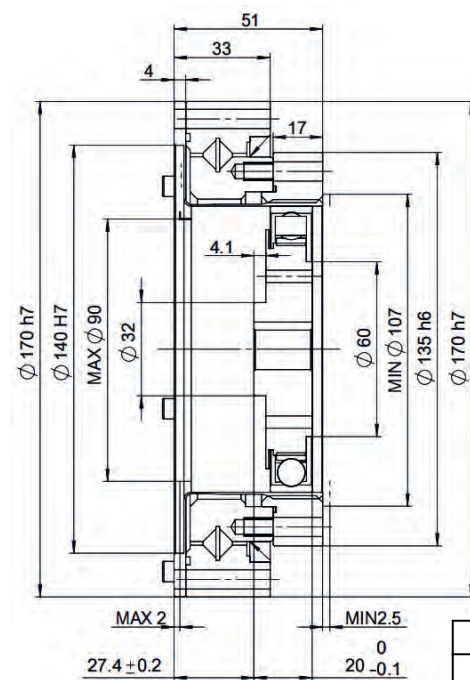
Full-section front view
