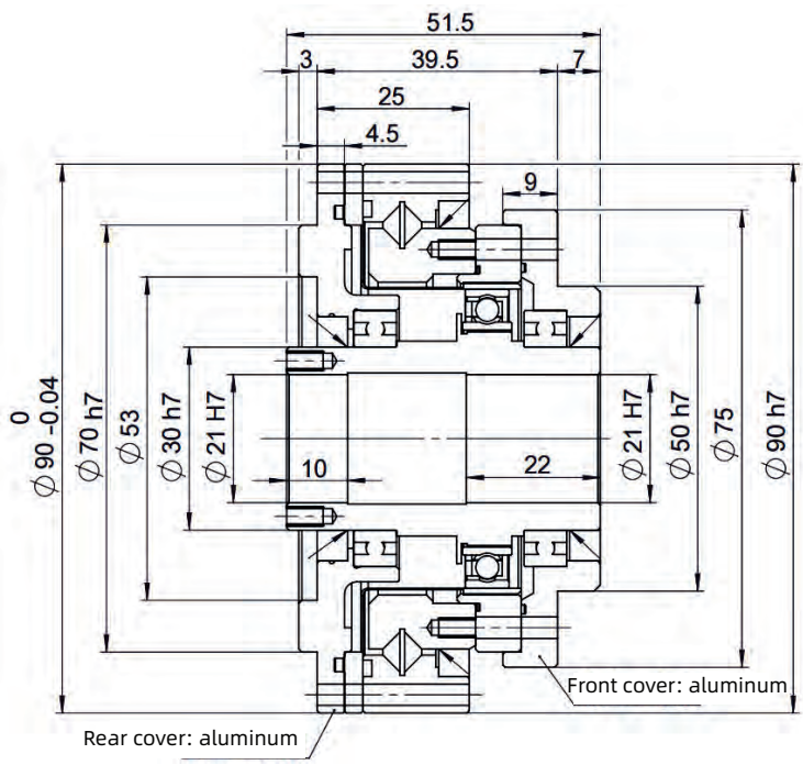
Full-section front view
