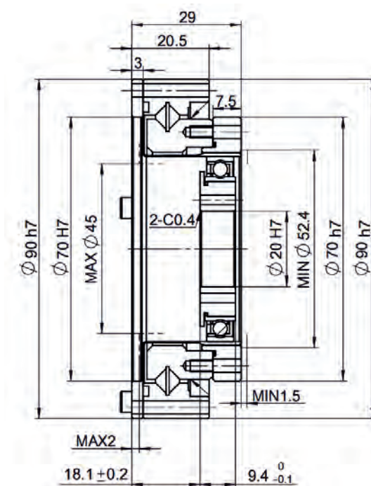
Full-section front view
