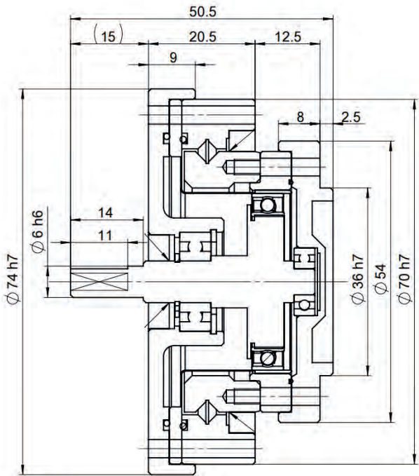
Full-section front view
